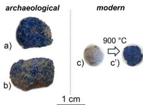
Fig. 1: Egyptian Blue archaeological samples (a, b) and modern synthesis before (c) and after (c') firing in muffle at 900 °C.
