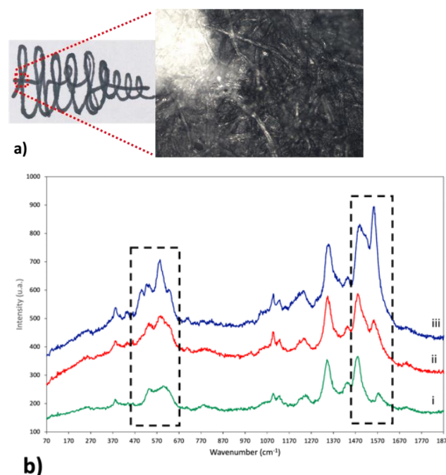
Figure 1. a) Visible image of a laboratory sample made with logwood ink, crossed out with a stroke of iron-gall ink, and magnified 10X around the overlapping area where the Raman mapping analysis was performed. b) Raman spectra excited at 638 nm of (i) iron-gall ink, (ii) iron-gall ink on logwood ink, and (iii) logwood ink.
