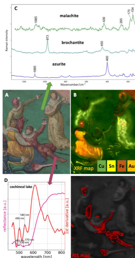
Fig. 1. Analysis of a fragment of the Hans Bol's miniature (1584). (A) macro-photography (1.6 x 1.2cm); (B) Macro-XRF map presenting the distribution of Cu, Au, Fe, and Sn; (C) Raman spectra of various pigments found in a green colored area; (D) RIS spectra of cochineal lake along with its distribution map.
