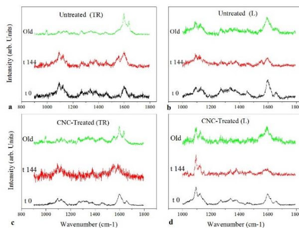
Fig. 1: Raman spectra acquired on untreated and CNC-treated samples.
