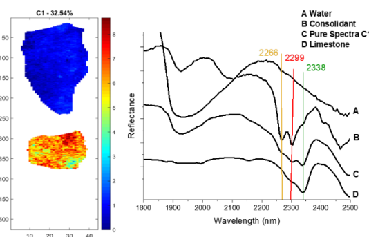
Fig 2: (left) Distribution map of the first component obtained by MCR that discriminates an untreated sample from a consolidated one and (right) the NIR spectra obtained by hyperspectral imaging.
