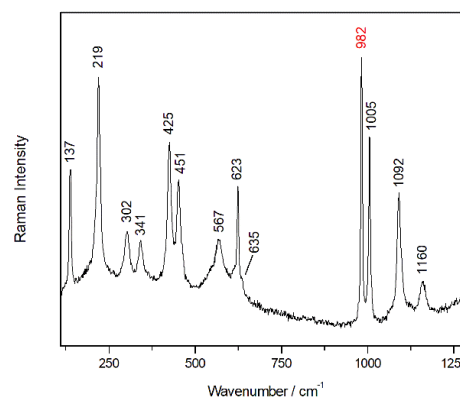
Fig. 1: Raman spectrum recorded on the dagger microfragments shows the presence of ammoniojarosite (in black) and epsomite (in red)
