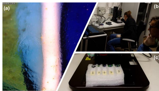
Fig. 1: Working on-site: (a) Detail of polichrome glass-gem from Aquileia (Museo Archeologico Nazionale di Aquileia), observed by the digital microscopy during one of the on-site characterisation campaigns, showing Blue, White, Light Blue and yellowish Green colors [catalogue ref. 48446]; (b) The Renishaw VIRSA™ Raman system's set up at the museum; (c) detail of several glass-gems ready for the Raman analysis.
