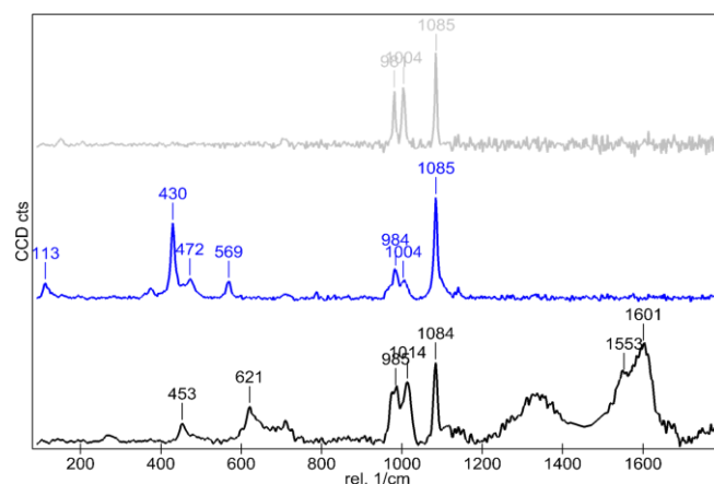
Fig. 1: Confocal Raman spectroscopy on a Roman Fresco (top) and resulting spectra (bottom).
