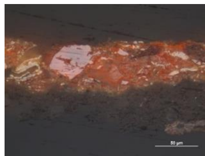
Fig. 1: Sample M-I2, large x-ray amorphous particle of orpiment glass. To the left of this particle is a crystal of natural orpiment exhibiting thin-foliated and kinked fragments. Vertically reflected light, 500x magnification.
