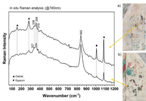
Fig. 1: Raman spectra collected in in situ with B&W Tek i-Raman® Plus spectrometer (Metrohm group) of crocoite ( \nu_4 327, 338, 358, 378 \text{cm}^{-1} , \nu_4 840 \text{cm}^{-1} ) on the southern wall paintings of former Cloister of Brandenburg Cathedral: bay 7, eastern part (a) and bay 6, western part (b). Contours of the figures are displayed to improve their readability.
