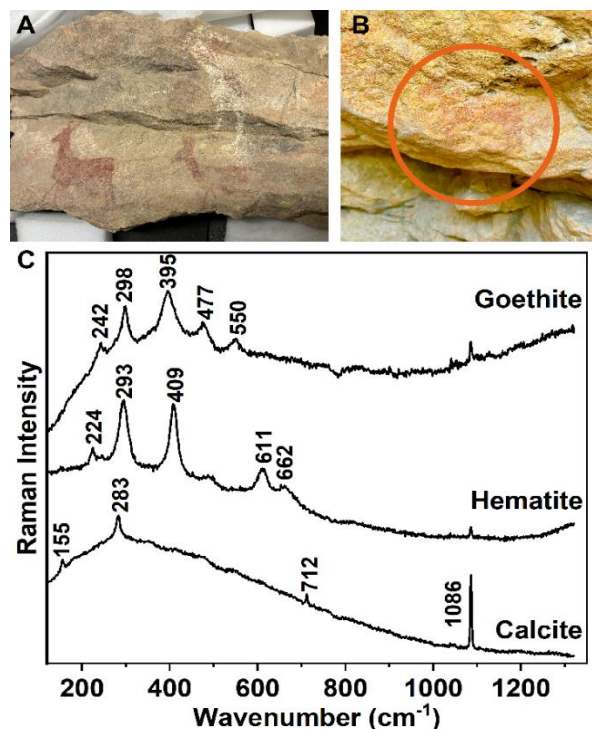
Fig. 1: (A) One of the blocks detached from the rock shelter; (B) Goat figure from rock art in the rock shelter of Minglanilla; (C) Raman spectra of goethite, hematite and calcite.
