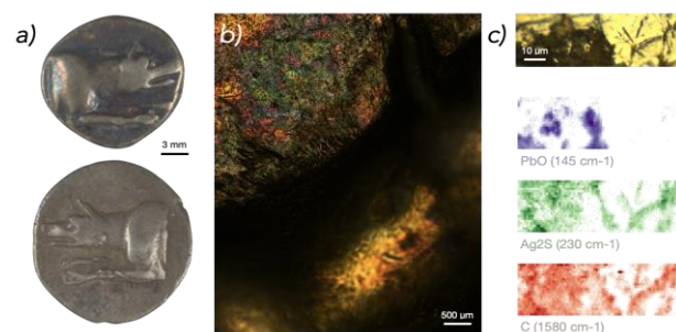
Fig. 1: a) Two silver coins with different patinas (the upper one has probably been electrolysed), b) microscope image of the upper coin's surface, c) \mu -Raman cartography of corrosion products on another coin's surface. The colour scales go from white (min) to intense shade (max).
