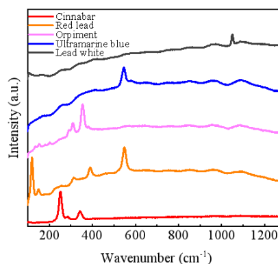
Fig. 2: A part of the Raman spectra measured in situ.
