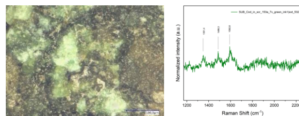
Fig. 1: Left: Microscopic image of a degraded copper-based pigment surface (Keyence digital microscope, Rx100 x700, full coaxial, fine depth composition with 1\text{ }\mu\text{m} step). Right: Raman spectrum obtained on the same pigment, acquired with the 532 nm laser in the extended mode, baseline corrected.
