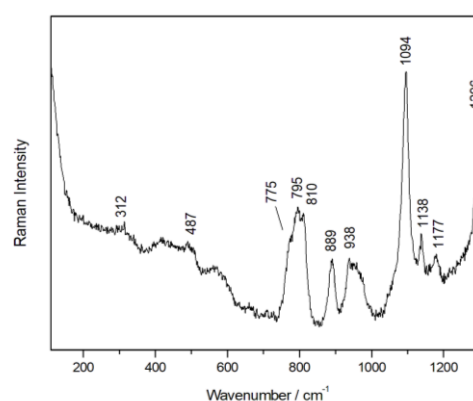
Fig 1: Raman spectra of the nanoparticle-based consolidant used to consolidate both the sandstone and the marly limestones.
