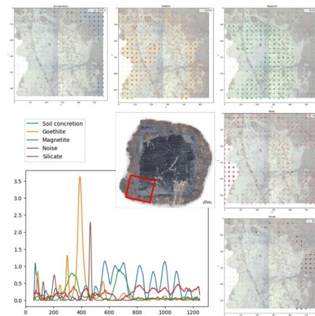
Fig. 1: Visualisation of the NMF results for 1 map on a nail cross-section. Components were found for: blue) poor Raman signal on soil concretion, yellow) Main bends for goethite, Green) Main bends for magnetite, Red) Noise, Brown) Main bends of silicate representing sand inclusions.
