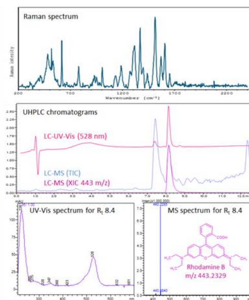
Fig. 1 Multidisciplinary analysis of red Rhodia pen.
