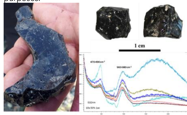
Fig. 1: Vitreous lead slag. Black tesserae. Raman spectra of black tesserae.
